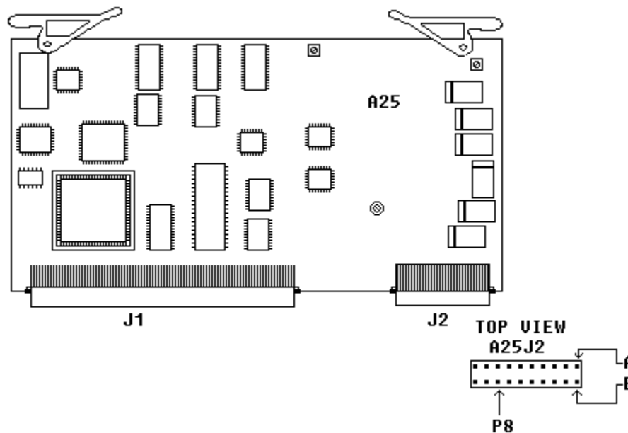
Figure 4. A25 digitizer module.
