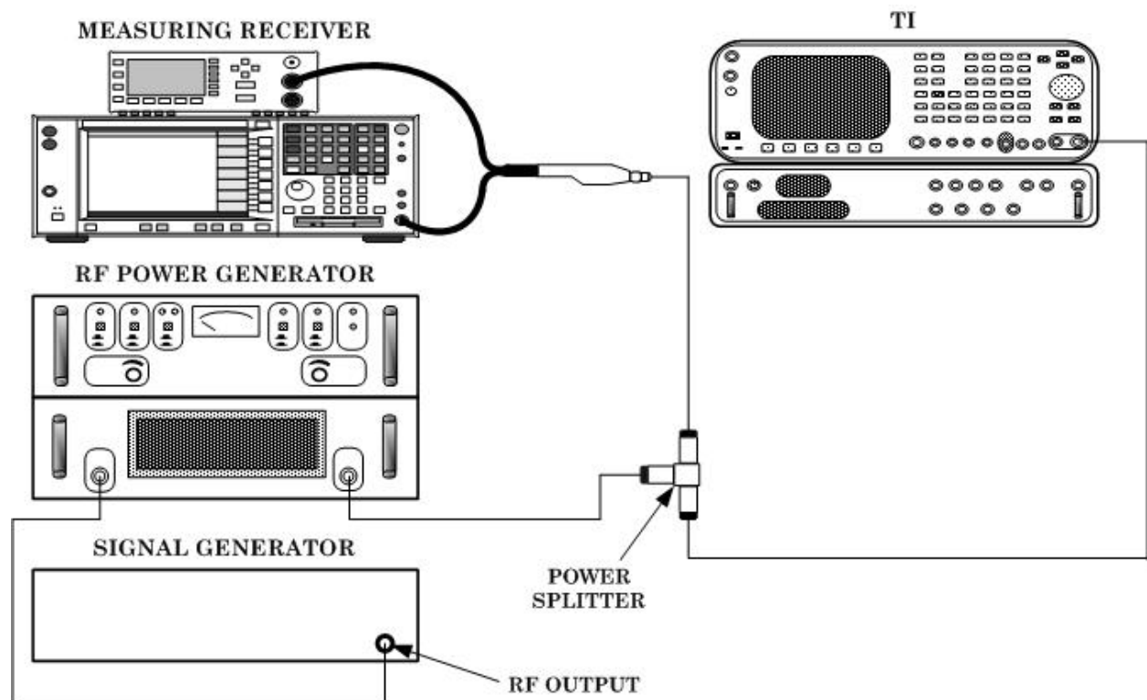
Figure 6. Power meter setup (20mW – 500mW range).
